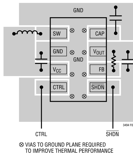
Figure 4. Recommended Layout
